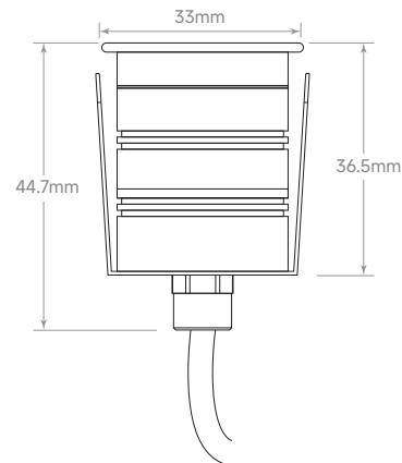
Lamp body's size
